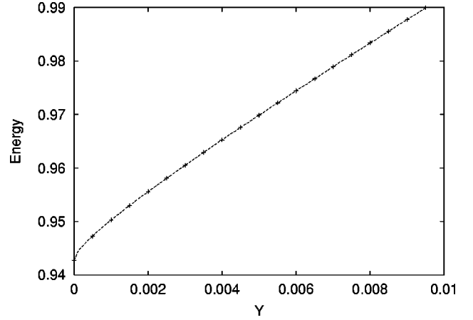
FIG. 1. The energy of the sphaleron configuration relative to the vacuum energy. The plusses are the values obtained by the extremization method. The solid curve denotes the least-squares fit to the form a + b\sqrt{\mathcal{Y}} + c\mathcal{Y} .
